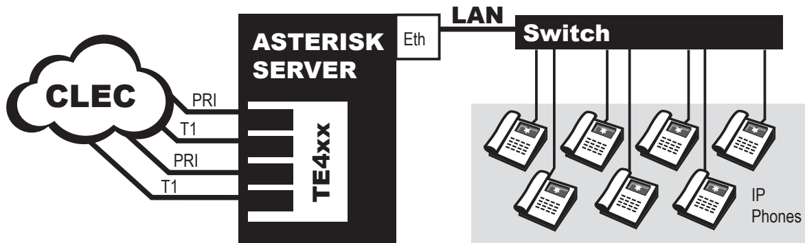
Figure 3: Sample IP Phone Application
