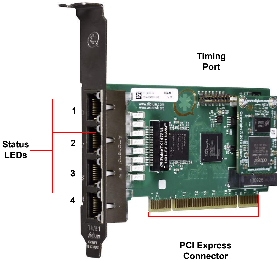
Figure 5: TE436B Card
