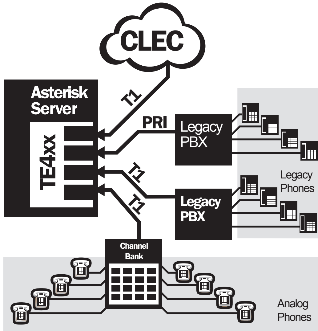
Figure 1: Sample Legacy Phone Application
