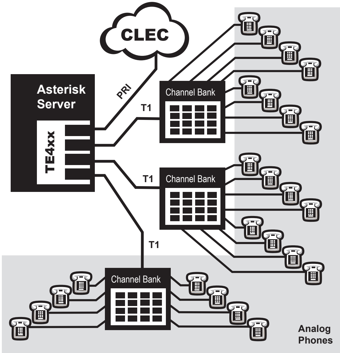
Figure 2: Sample Channel Bank Application
